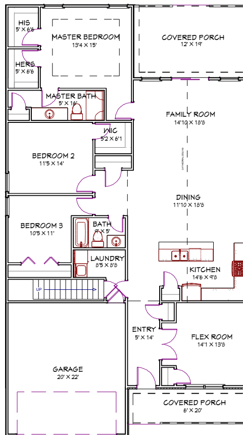
MAGNOLIA MAIN LEVEL FLOOR PLAN 2034 SF
